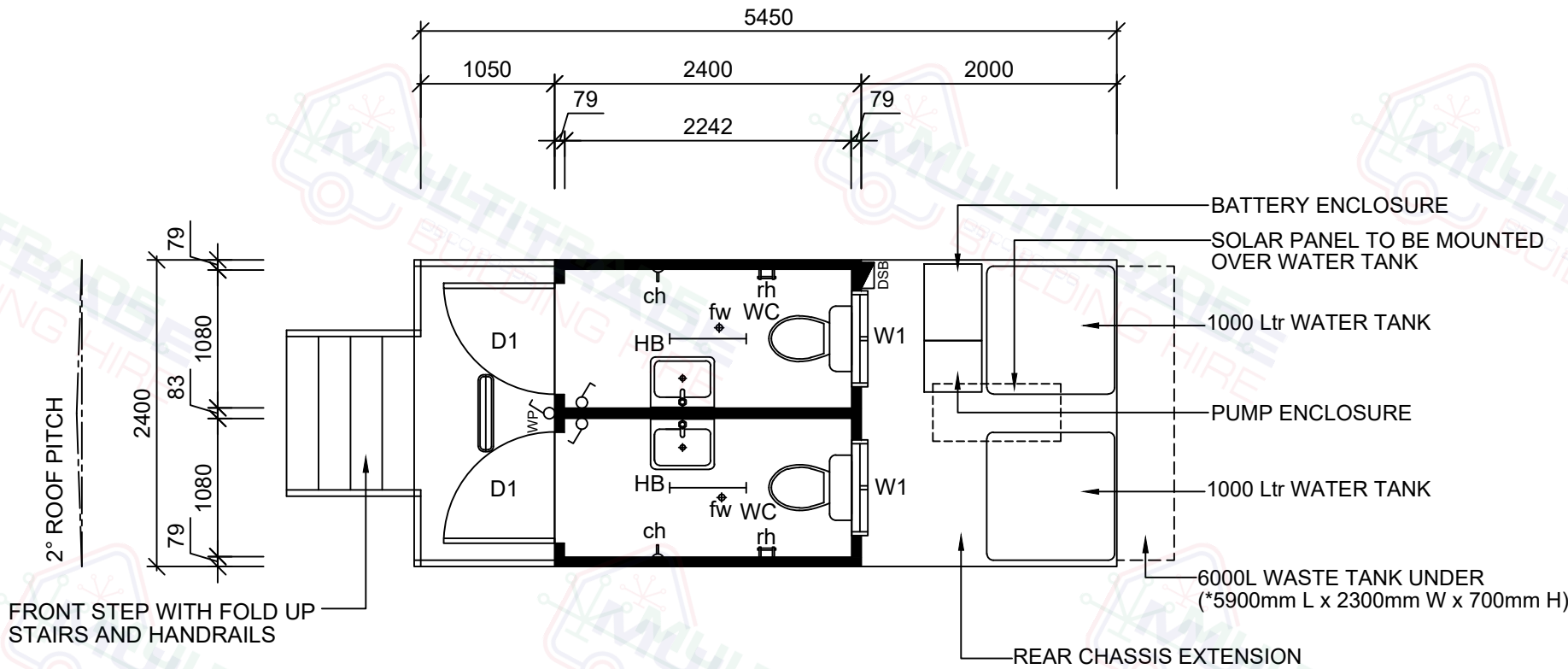
5.45x2.4m Solar Toilet / 6000L Waste Tank - Floor Plan
